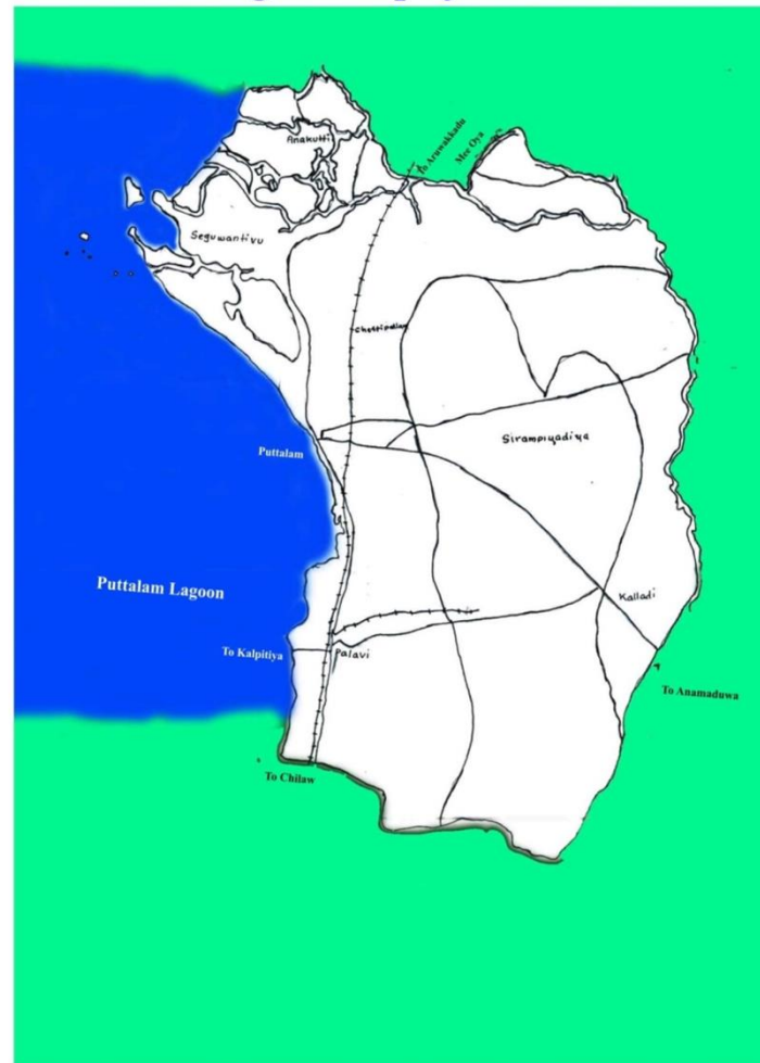
Geological Map of Puttalam.
